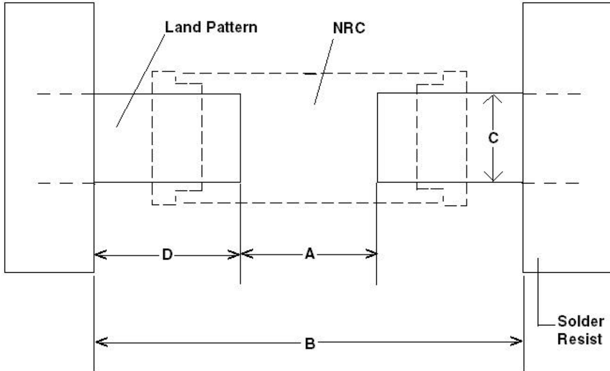
SOLDERING LAND PATTERN DIMENSIONS (mm)
