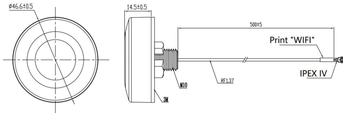
NANE46X14PJW2C500A1F Dimensions
