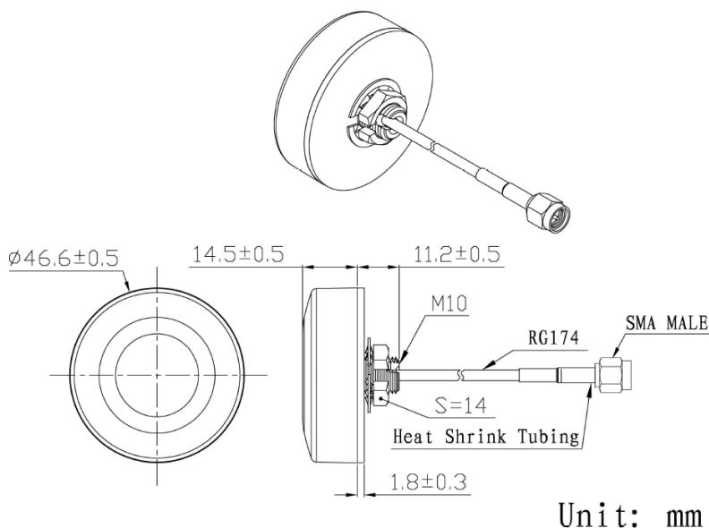
NANE46X14PJW2C302A0F Dimensions
