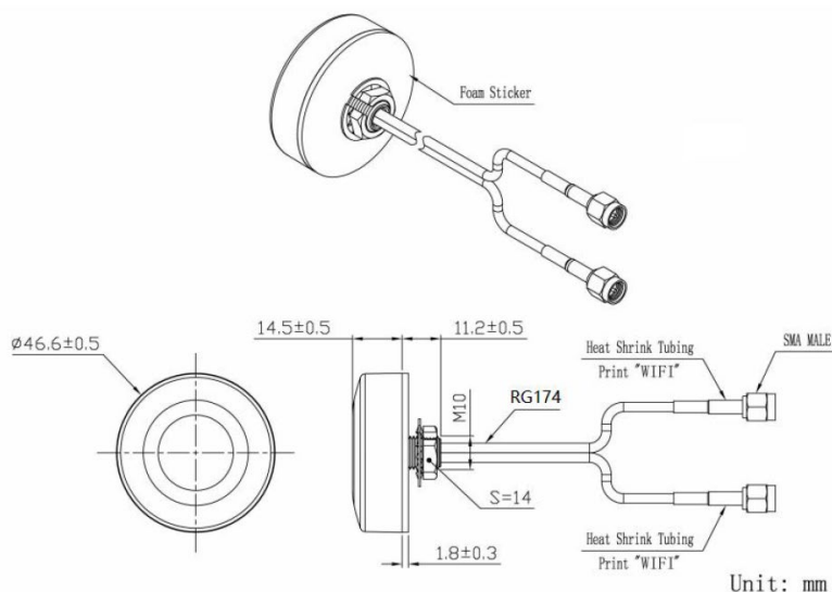
NANE46X14PJW2C102A0F Dimensions
