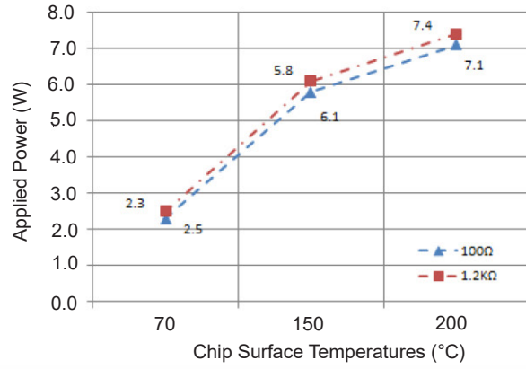
NTRN10 Chip Temperature vs. Applied Power
