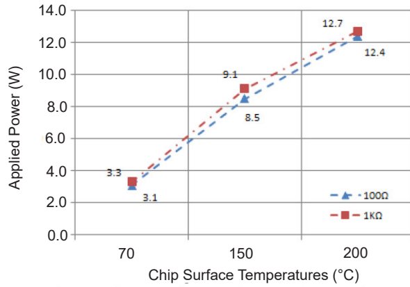
NTRN25 Chip Temperature vs. Applied Power
