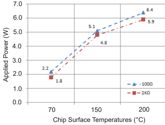
NTRN06 Chip Temperature vs. Applied Power
