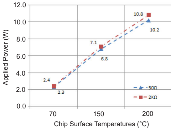
NTRN12 Chip Temperature vs. Applied Power
