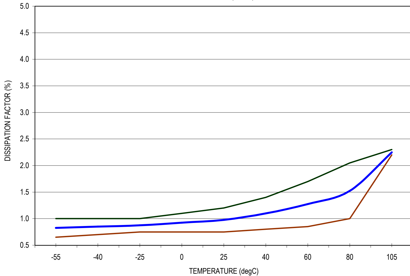
NSP SERIES TYPICAL DISSIPATION FACTOR (120Hz) OVER TEMPERATURE
