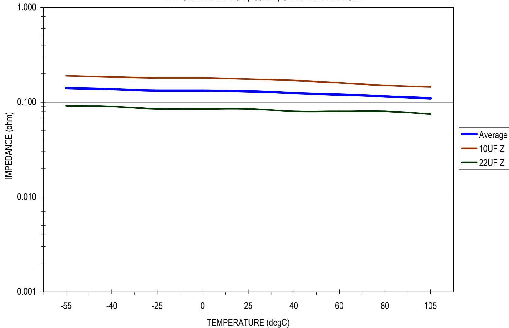
NSP SERIES TYPICAL IMPEDANCE (100KHz) OVER TEMPERATURE
