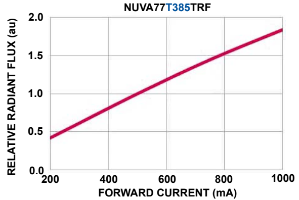
FORWARD CURRENT VS. RELATIVE RADIANT FLUX @ +25°C
