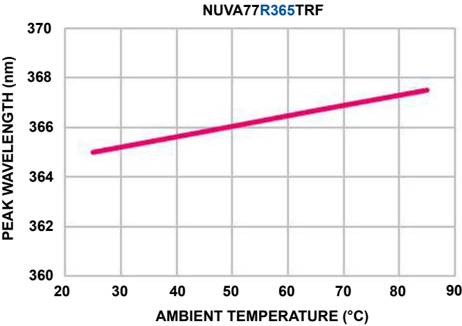
AMBIENT TEMPERATURE VS. PEAK WAVELENGTH @ 500mA If
