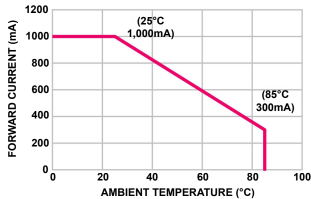
TEMPERATURE DERATING CURVE ( T_j < 130^\circ\text{C} , \sim 32^\circ\text{C/W} ) (Ambient Temperature vs. Allowable Forward Current)
