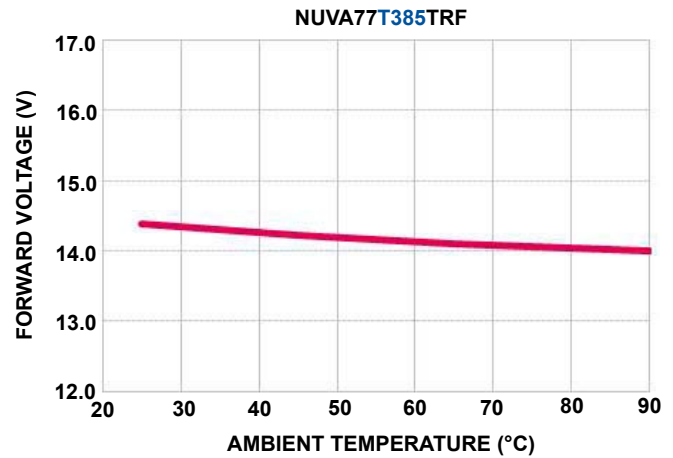
AMBIENT TEMPERATURE VS. FORWARD VOLTAGE @ 500mA If
