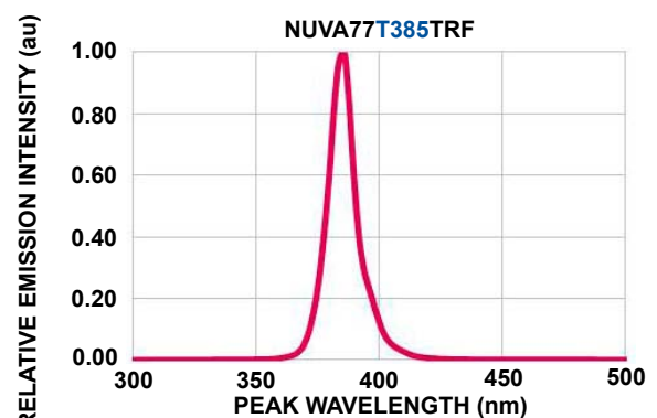
SPECTRUM @ +25°C & 500mA
