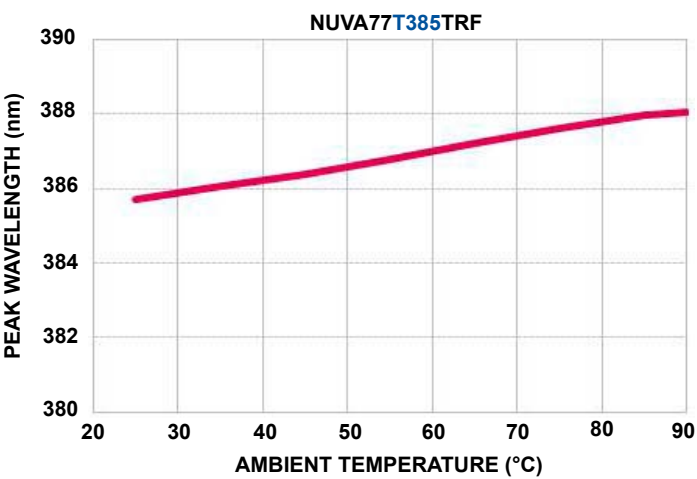
AMBIENT TEMPERATURE VS. PEAK WAVELENGTH @ 500mA If
