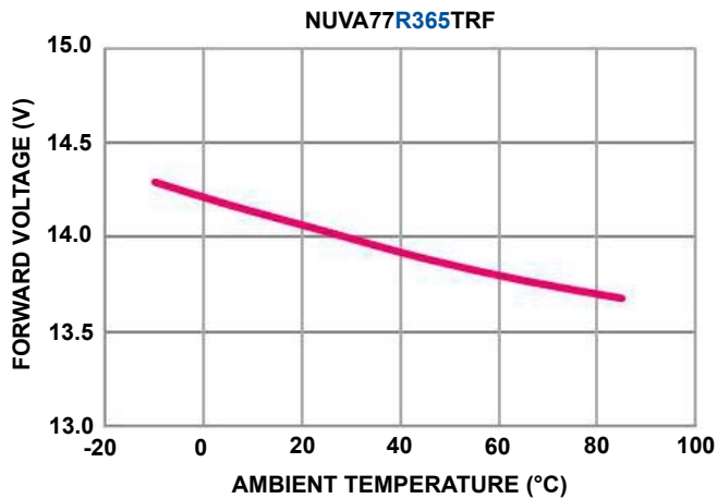
AMBIENT TEMPERATURE VS. FORWARD VOLTAGE @ 500mA If
