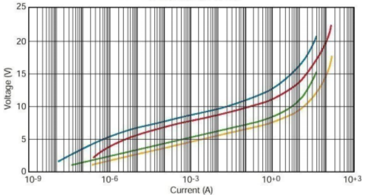
VI Curves: 10V & 15V
