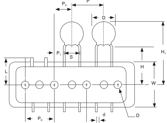
Straight Leads >12 \sim 23 mm diameter (a slight lead flare may be present)
