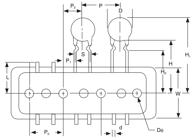
Crimped Leads >12 \sim 23 mm diameter Inward (J) & Outward (K) are available
