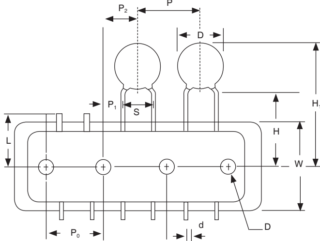
Straight Leads \leq 12 mm diameter (a slight lead flare may be present)
