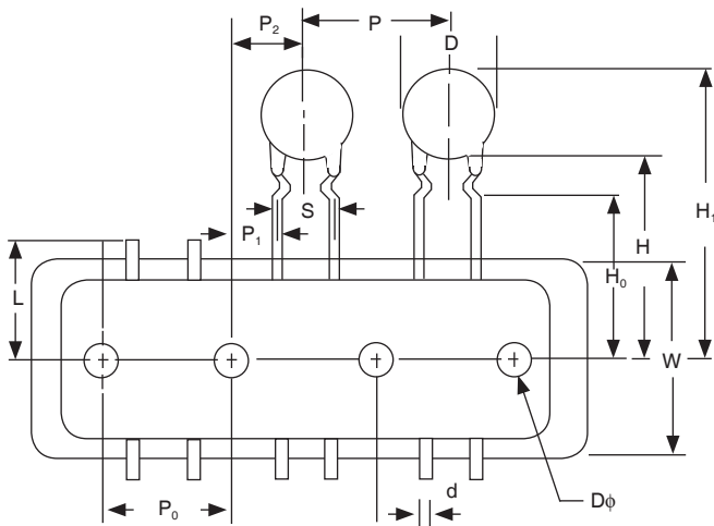
Crimped Leads \leq 12 mm diameter Inward (J) & Outward (K) are available
