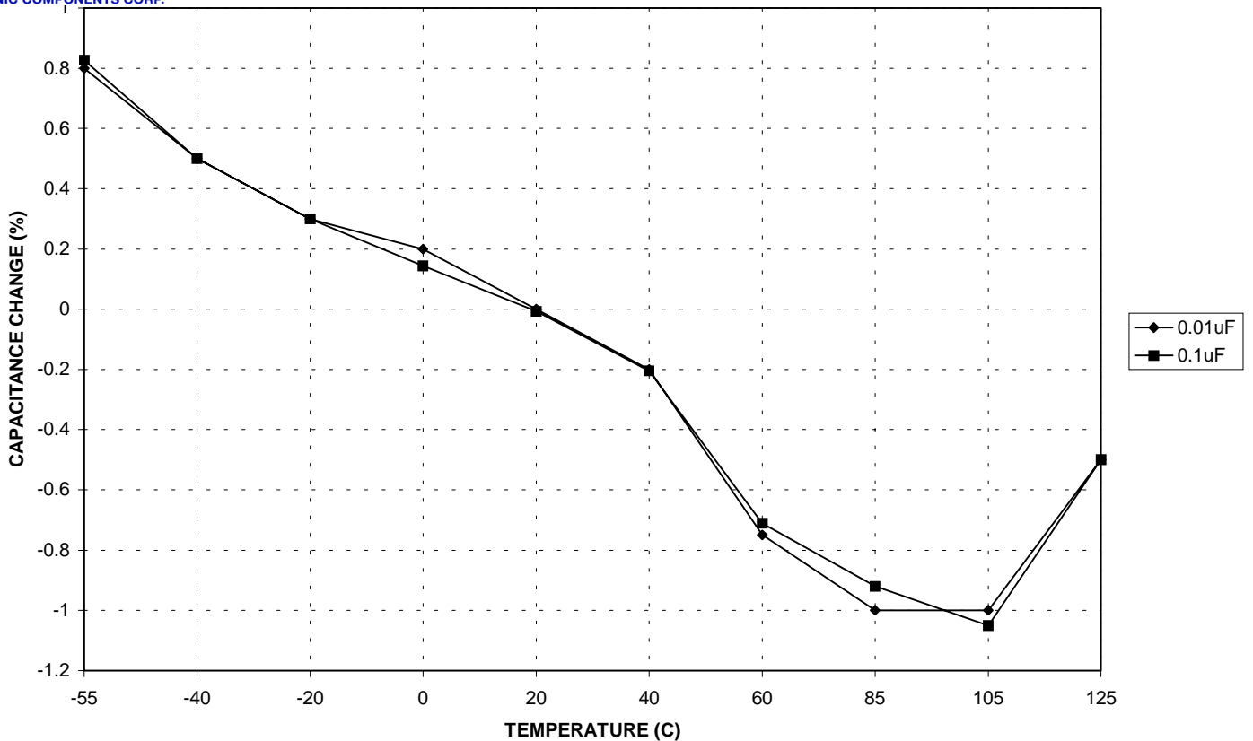
TYP. TEMP CHARACTERISTICS OF NSPC SERIES.
