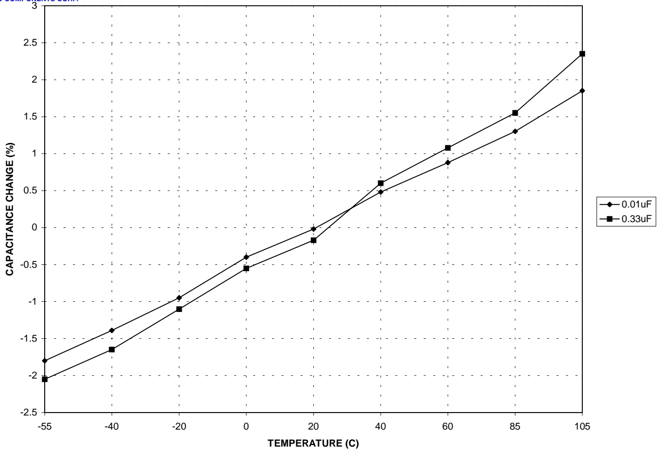
TYP. TEMP CHARACTERISTICS OF NSFC SERIES.
