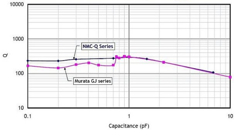
0402 size NP0 Q level comparison @ 3GHz
