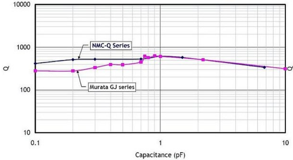
0402 size NP0 Q level comparison @ 2GHz
