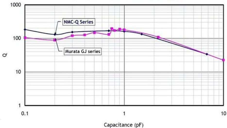
0402 size NP0 Q level comparison @ 3GHz
